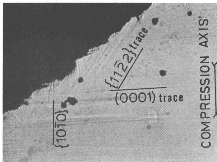
Fig. 6 - Pyramidal Slip Lines on (11\bar{2}0) Surface Shown in Figure 2 at F Match \{11\bar{2}2\} Trace for this Surface. Mag. 240X
